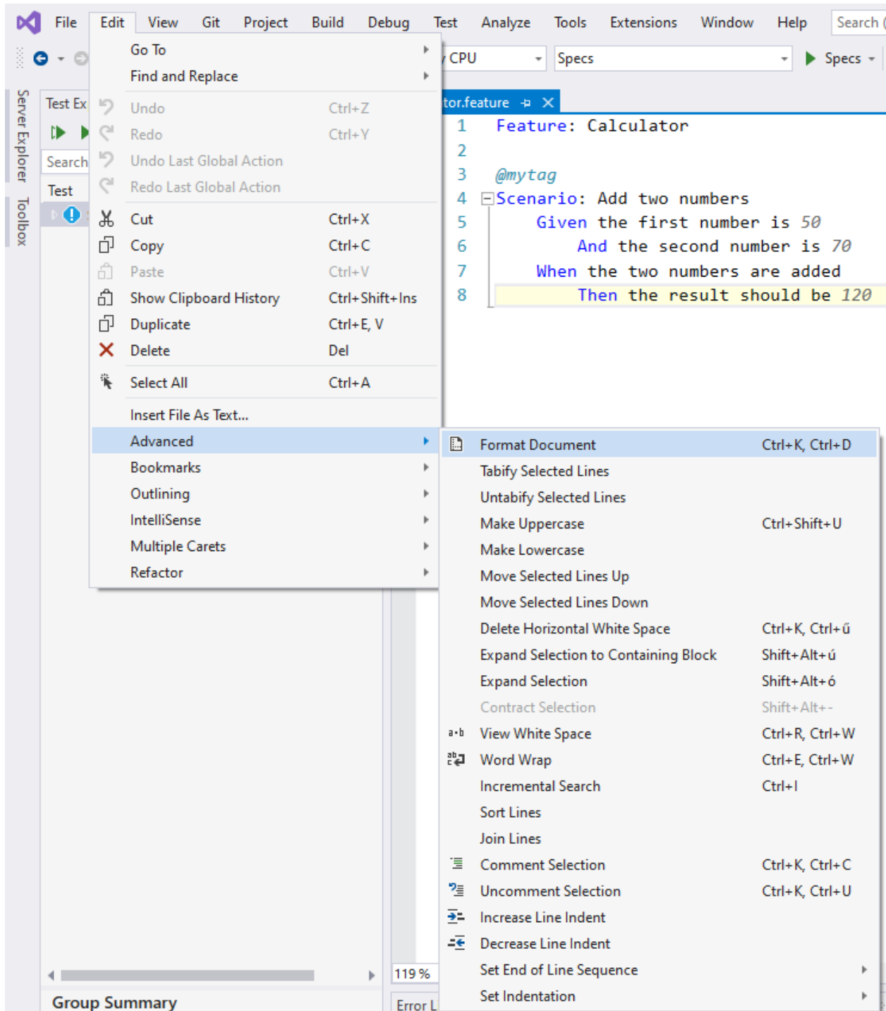
Fig. 4: Format document
